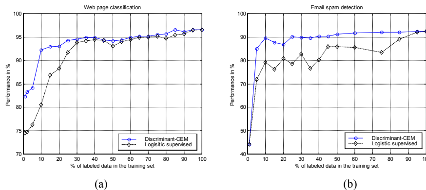
Fig. 1. Web Pages classification (a) and e-mail Spam detection (b) - Performance of two classifiers with respect to the ratio x of labeled data in the training set. The classifier is a logistic unit trained with labeled data in a supervised scheme (dashed bottom curves) and using the semi-supervised discriminant-CEM algorithm (solid top curves)
