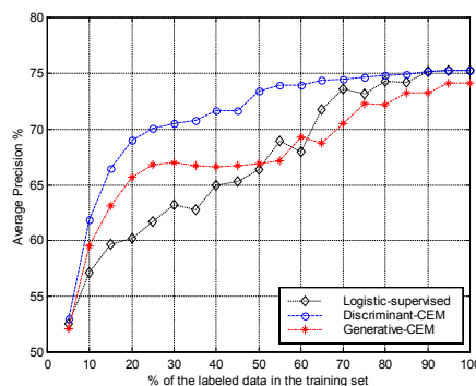
Fig. 2. Average precision of 3 trainable summarizers with respect to the ratio of labeled sentences in the training set for the cmp_lg collection
