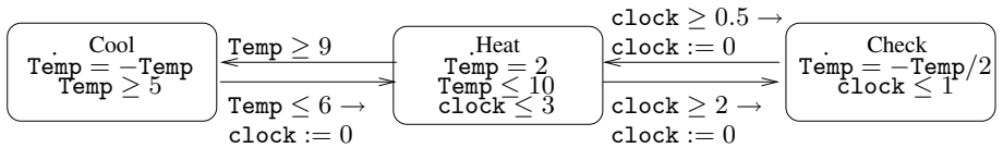
Fig. 3. The Thermostat example. We omit the differential equation \dot{\text{clock}} = 1 in all three locations.
