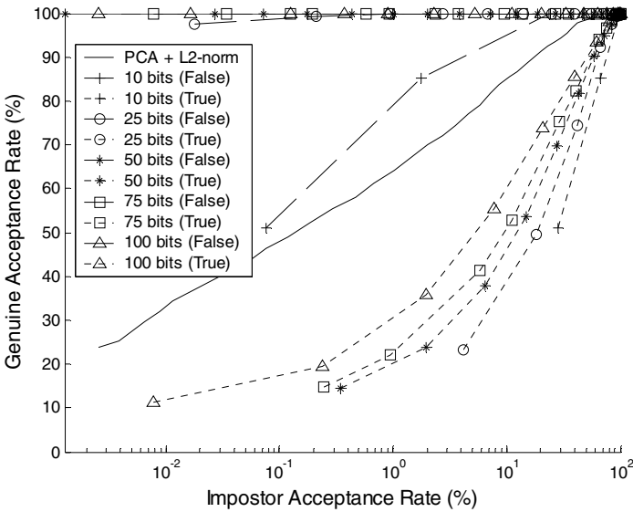
Fig. 4. ROC curves of various dimensions of FaceHash under different assumptions
