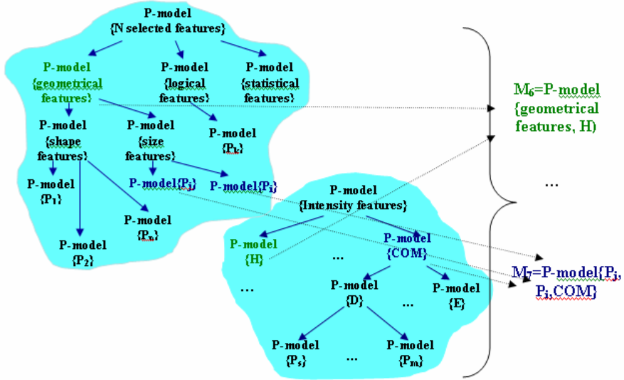
Fig. 4. Generating Descriptive Trees
