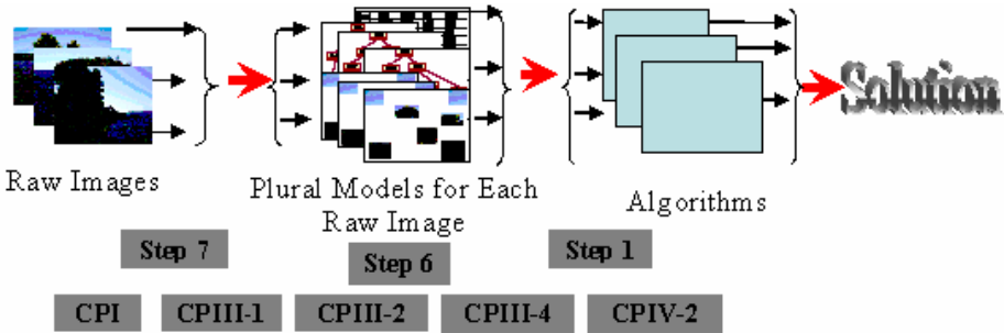
Fig. 3. Image recognition. General case (multiple classifiers and model plurality)
