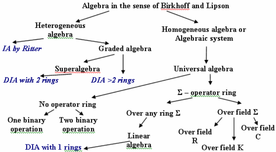
Fig. 6. Hierarchy of algebras
