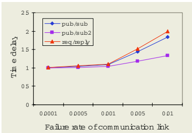
Fig. 2. Time delay per transaction links ( \alpha=0.5, s(n)=1, t_{ps}=1, t_{rr}=1, \mu=0.1, \text{ and } \beta=0.5 for pub/sub and req/reply and \beta=0.2 for pub/sub2)
