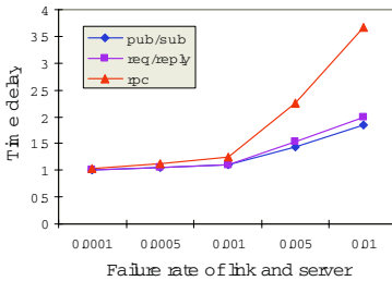
Fig. 4. Time delays per transaction ( \alpha=0.5, t_{ps}=1, t_{rr}=1, t_{poll}=1, \beta=0.5, \mu=0.1, \mu_s=0.1 )
