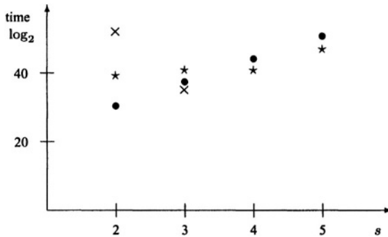
Figure 7. Time-complexity for the main loop ( \bullet ), SearchForParallelFlats ( \star ), and the combine-method ( \times ) for dimension n = 16 and varying s
