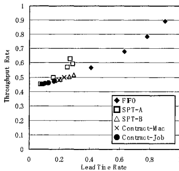
Figure 3 Large lot size manufacturing (Lead time-Throughput) L=3, Kind=3, Kn=1, SimTime=3600, ProcTime(50,10), SetUpTime(Mp,Vp): Mp=\{20,40,60,80,100\}, Vp=\{4,8,12,16,20\}, ArrivalTime=50, Lot=3, BiddingPeriod=0
