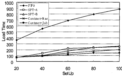
Figure 1 Large lot size manufacturing (Lead Time) L=3, Kind=3, Kn=1, SimTime=3600, ProcTime(50,10), SetUpTime(Mp,Vp): Mp=\{20,40,60,80,100\}, Vp=\{4,8,12,16,20\}, ArrivalTime=50, Lot=3, BiddingPeriod=0
