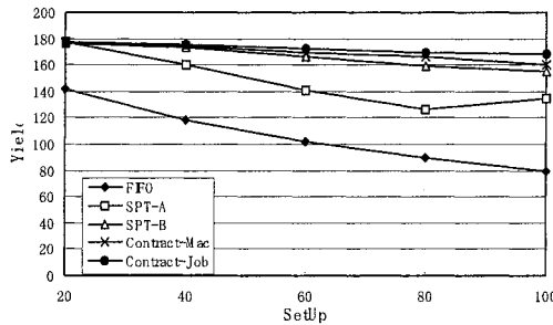
Figure 2 Large lot size manufacturing (Yield) L=3, Kind=3, Kn=1, SimTime=3600, ProcTime(50,10), SetUpTime(Mp,Vp): Mp=\{20,40,60,80,100\}, Vp=\{4,8,12,16,20\}, ArrivalTime=50, Lot=3, BiddingPeriod=0
