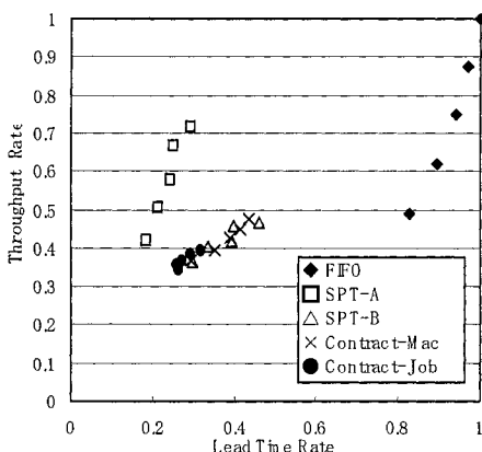
Figure 4 Small lot size manufacturing (Lead time-Throughput) L=3, Kind=30, Kn=1, SimTime=3600, ProcTime(50,10), SetUpTime(Mp,Vp): Mp=\{20,40,60,80,100\}, Vp=\{4,8,12,16,20\}, ArrivalTime=50, Lot=3, BiddingPeriod=0
