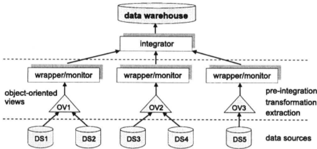
Figure 1. The application of object-oriented views in a data warehouse architecture
