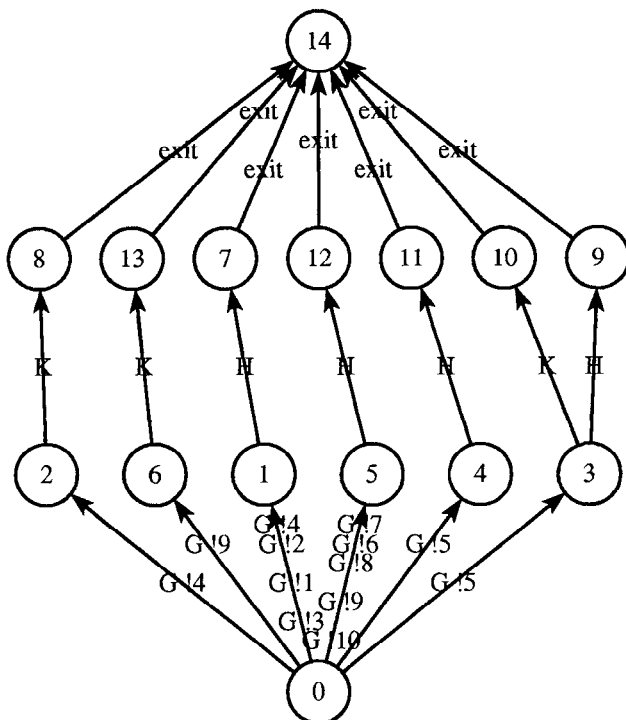
Figure 2. Binary Coded Graph for process P
