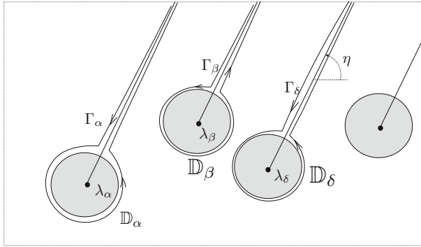
Fig. 4 The paths of integration \Gamma_\alpha, \Gamma_\beta , etc \alpha, \beta, \dots \in \{1, \dots, s\}
