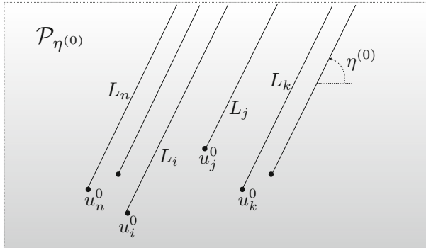
Fig. 2 The poles u_j^0, 1 \leq j \leq n , of system (2.26) and plane \mathcal{P}_{\eta^{(0)}} with branch cuts L_j
