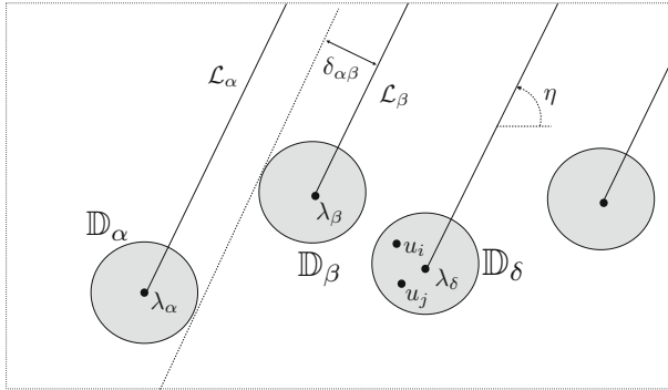
Fig. 3 The figure represents the half lines \mathcal{L}_\alpha, \mathcal{L}_\beta , etc, for \alpha, \beta, \dots \in \{1, \dots, s\} , in direction \eta = 3\pi/2 - \tau , the discs centred at the coordinates \lambda_1, \dots, \lambda_s of the coalescence point u^c , and the distances \delta_{\alpha\beta} . Also two points u_i, u_j are represented, such that u_i^c = u_j^c = \lambda_\delta for some \delta \in \{1, \dots, s\} . Important: now \eta refers to u^c , differently from Sect. 2.2 and Fig. 2
