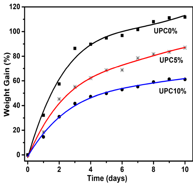
Fig. 9 Water absorption of UPC0, UPC5, and UPC10
