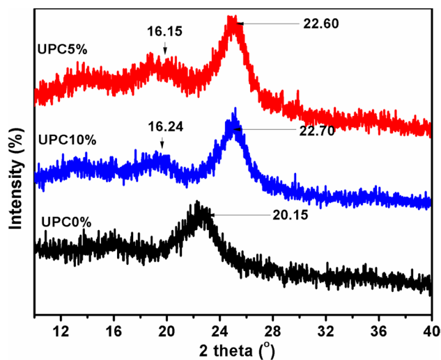
Fig. 10 XRD diffractograms of non-woven/fabric jute composites UPC0, UPC5 and UPC10
