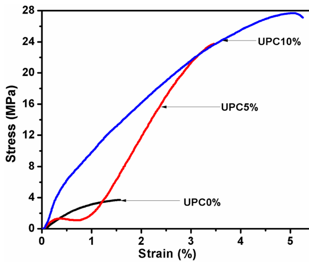
Fig. 7 Stress–strain curves
