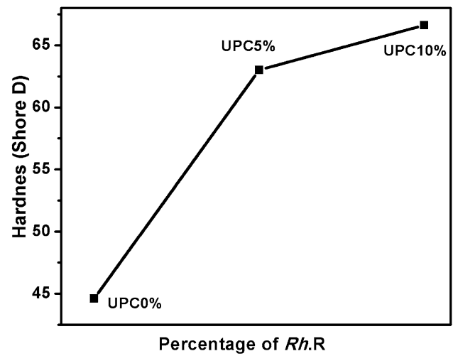
Fig. 8 Relationship between hardness shore D versus alkyd resin content in UP blend
