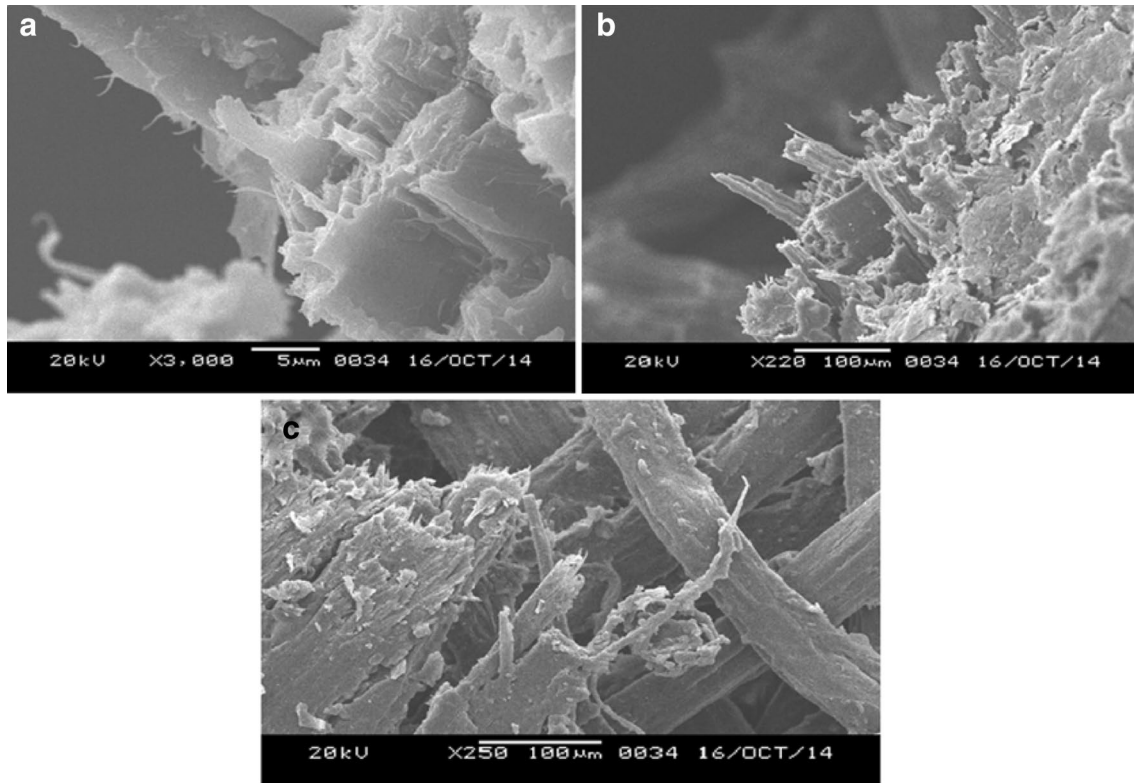
Fig. 5 Fracture surface of a UPC10, b UPC5, and c UPC0
