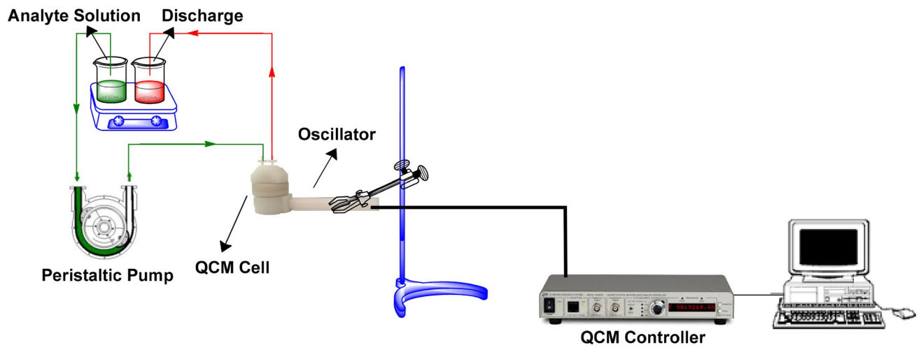
Fig. 2 Representation of QCM sensing system
