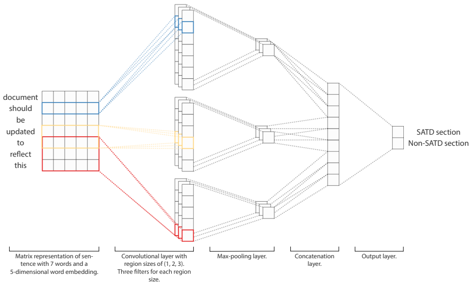
Fig. 2 Architecture of the CNN model
