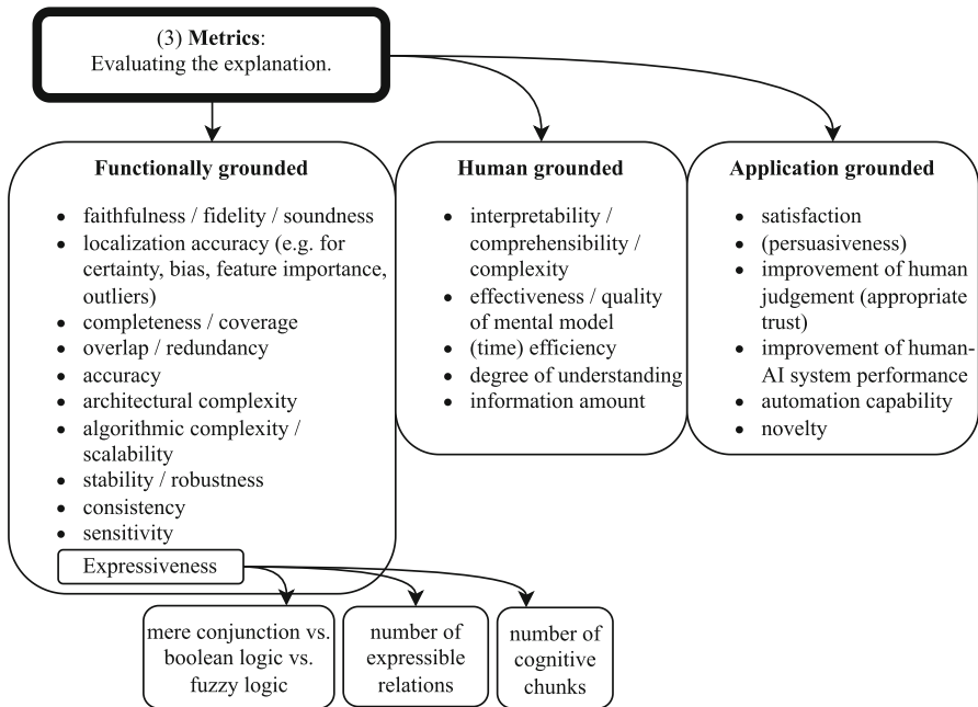
Fig. 6 Overview of the XAI metrics detailed in Sect. 5.3. Find a visualization of the complete taxonomy in Fig. 7
