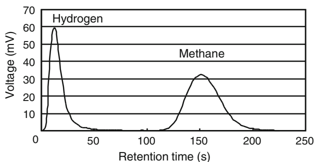
Fig. 2 Chromatogram for a mixture of 10 ppm hydrogen and 1000 ppm methane
