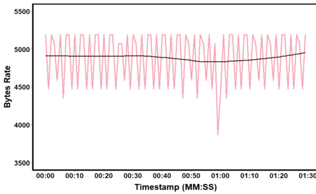
Fig. 6 Constant low rate RDoS attack byte rate
