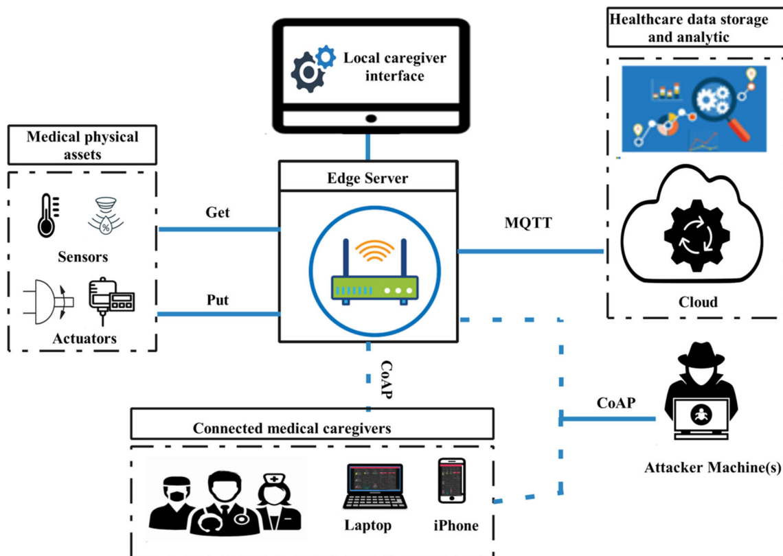
Fig. 4 Testbed architecture
