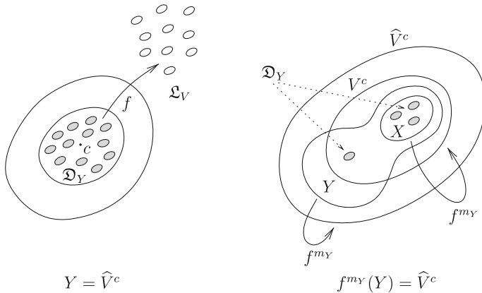
Fig. 1. On the left, the family associated to a connected component Y of \widehat{V} ; on the right, the one associated to a higher order pull-back Y of \widehat{V}
