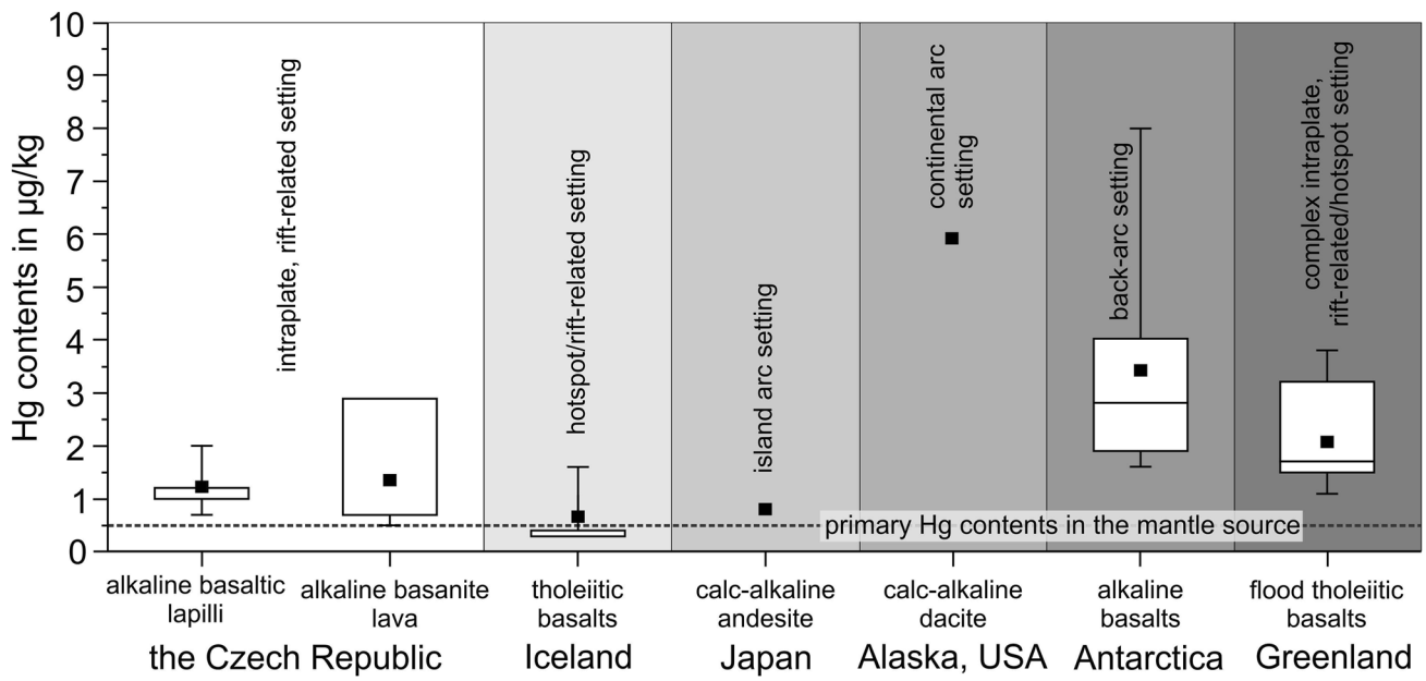
Fig. 2 Hg contents in volcanic rocks from different geotectonic settings. Data for Antarctica and Greenland were taken from Coufalík et al. (2015)
