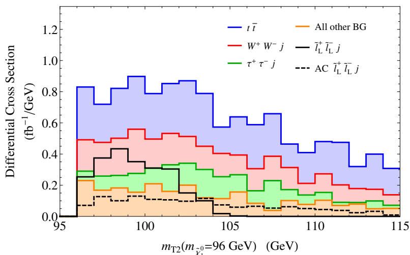
Figure 5. m_{T2}(m_{\tilde{\chi}_1^0}) distribution after cuts 1–7 for backgrounds (histograms stacked) and signal using m_{\tilde{\chi}_1^0} = 96 GeV for both. Note that the vertical axis is not log-scaled. Two different signal scenarios are shown: degenerate left-handed selectrons and smuons with mass m_{\tilde{l}_L} = 104 GeV each decaying to a lepton plus either a 96 GeV neutralino LSP (solid black) or an auto-concealed modulino KK-tower (dashed black). When scanning the (m_{\tilde{l}}, m_{\tilde{\chi}_1^0}) plane the expected signal and backgrounds at (m_{\tilde{l}}, m_{\tilde{\chi}_1^0}) = (104, 96) GeV are evaluated in step 8 using m_{T2}(96 \text{ GeV}) < 104 GeV. For the auto-concealed model, where multiple states play the role of LSP, we use three bins to evaluate the signal — m_{T2}(80 \text{ GeV}) , m_{T2}(88 \text{ GeV}) , m_{T2}(96 \text{ GeV}) < 104 \text{ GeV} — and choose the one with the largest signal significance.
