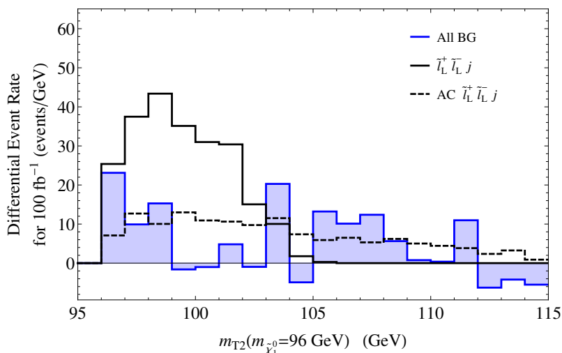
Figure 6. Different flavor subtracted m_{T2}(p_T^{l_1}, p_T^{l_2}; m_{\tilde{\chi}_1^0}) distribution after cuts 1–7 for backgrounds and signal using m_{\tilde{\chi}_1^0} = 96 GeV for both. Two different signal scenarios are shown: degenerate left-handed selectrons and smuons with mass m_{\tilde{l}_L} = 104 GeV each decaying to a lepton plus either a 96 GeV neutralino LSP (solid black) or an auto-concealed modulino KK-tower (dashed black). Backgrounds are subtracted as described in section 3.3. The results are shown in this figure, not including the m_{T2} cut described in step 8.
