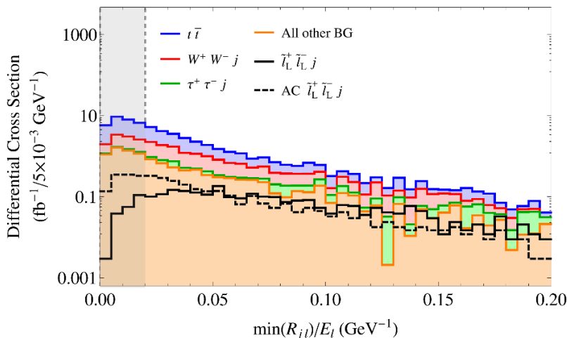
Figure 3. \min(R_{j_l})/E_l distributions after cuts 1–5 for backgrounds (histograms stacked) and two different signal scenarios: degenerate left-handed selectrons and smuons with mass m_{\tilde{l}_L} = 104 GeV each decaying to a lepton plus either a 96 GeV neutralino LSP (solid black) or an auto-concealed modulino KK-tower (dashed black). The gray area indicates the region removed in step 6 of the analysis.
