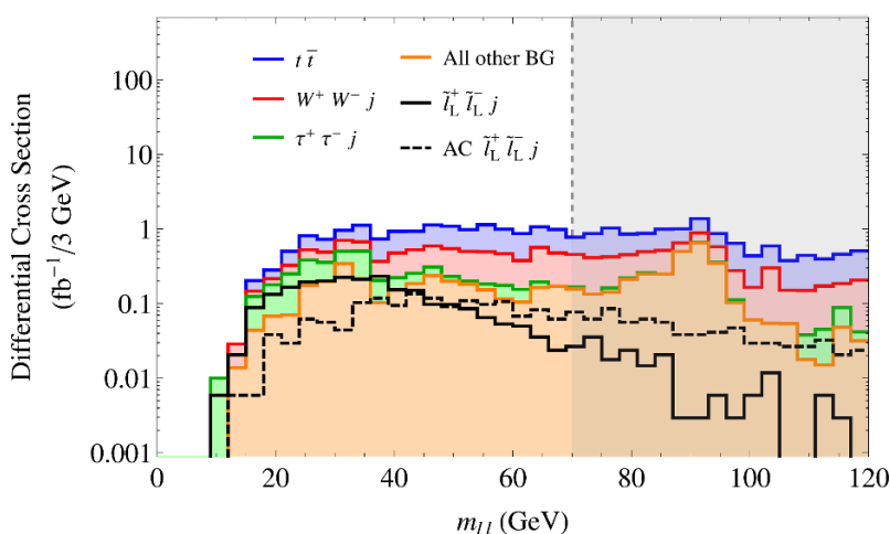
Figure 4. m_{ll} distributions after cuts 1–6 for backgrounds (histograms stacked) and two different signal scenarios: degenerate left-handed selectrons and smuons with mass m_{\tilde{l}_L} = 104 GeV each decaying to a lepton plus either a 96 GeV neutralino LSP (solid black) or an auto-concealed modulino KK-tower (dashed black). The gray area indicates the region removed in step 7 of the analysis.
