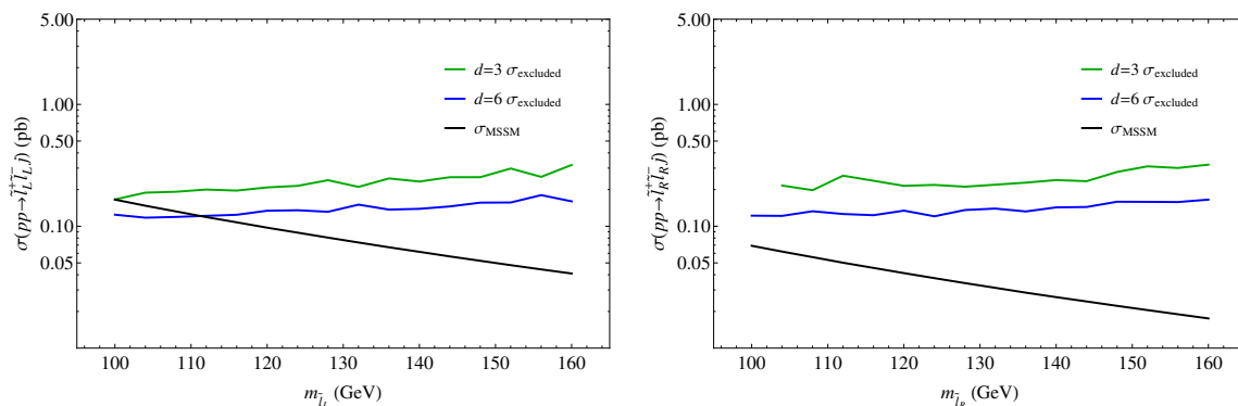
Figure 8. Potential 95% CL exclusion reach at LHC14 with 100\text{fb}^{-1} for the production cross section of auto-concealed sleptons decaying to a modulino KK-tower in d = 3 (green) or d = 6 (blue) extra dimensions for left-handed (left plot) or right-handed (right plot) sleptons. The black line shows the tree level production cross section for pp \rightarrow \tilde{l}^+ \tilde{l}^- j indicating that, with this amount of data, the LHC should be sensitive to left-handed sleptons for d = 6 (3) up to 110 (100) GeV. The production cross section of right-handed sleptons is smaller, requiring more data for sensitivity.
