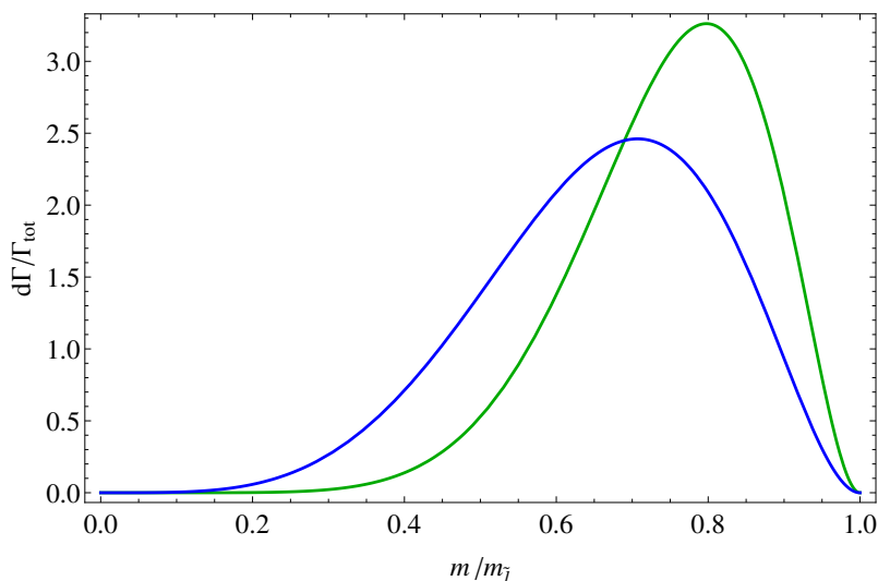
Figure 1. Differential decay rate for sleptons in an auto-concealed SUSY scenario. Here sleptons decay to the KK-tower of a bulk modulino LSP living in d = 6 (green) or d = 3 (blue) extra dimensions. The modulino mass is given as a ratio to the slepton mass m_{\tilde{l}} on the horizontal axis. Since the number of KK-modes grows like \sim m^{d-1} , the d = 6 scenario results in a more compressed spectrum.
