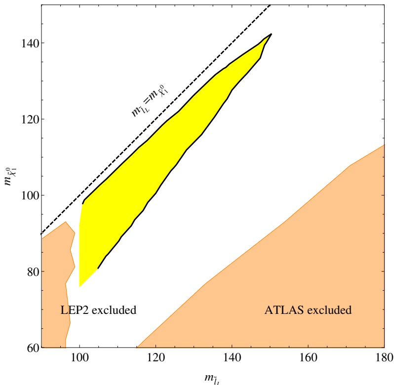
Figure 7. Potential 95% CL exclusion reach at LHC14 with 100 \text{ fb}^{-1} for degenerate left-handed smuons and selectrons. Yellow area indicates the region excluded by this analysis, while orange areas indicate regions already excluded by LEP2 [31, 32] and ATLAS [2].
