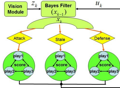
Fig. 6. Bayes Processing Flow Chart
