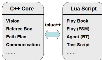
Fig. 9. Script architecture with Lua
