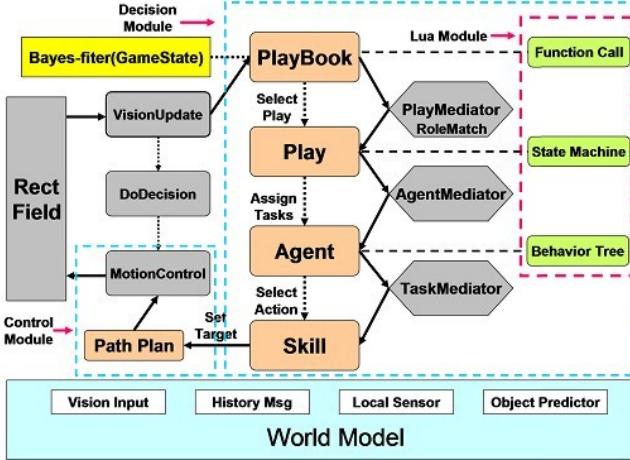
Fig. 3. Software architecture
