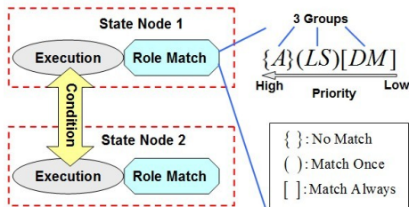
Fig. 7. FSM-based Role Match Framework. A role match item’s syntax is described on the right: the letter in the string is short for the role’s name in the state node (A-Assister, L-Leader, S-Special, D-Defender, M-Middle). We offer three modes for matching, No Match means to keep the role as same as last state, Match Once means match the role once stepping into this state, and Match Always means do role match every cycle. If a robot is missing, then ignoring the last role in the item and No Match group always has a higher priority.
