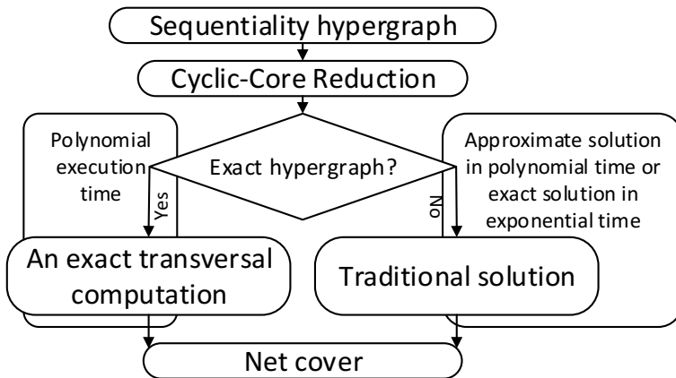
Fig. 1. Idea of exact transversal method
