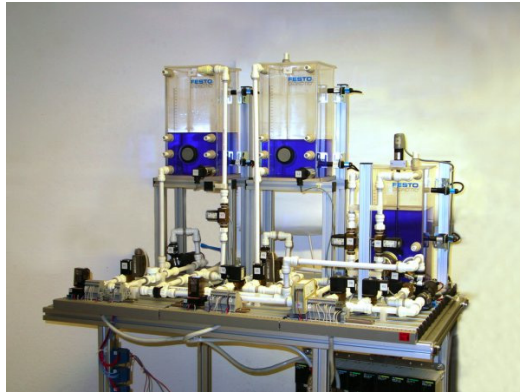
Fig. 6. Depiction of the process plant used in the case study
