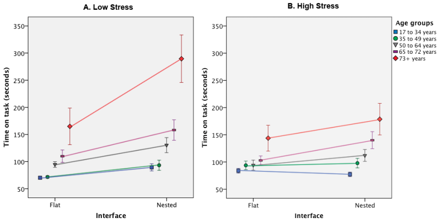
Fig. 5. Time to complete the task on flat and nested interfaces under A) Low stress and B) High stress condition
