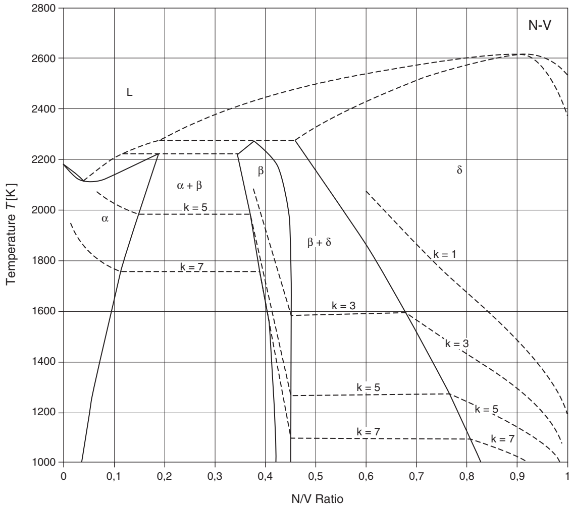
Fig. 1 N-V. An assessed Phase diagram of the N-V system [00Wan]. k indicates the N_2 pressure isobars; index k is p(N_2) = 10^{-k} bar
