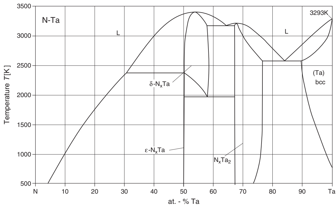
Fig. 1 N-Ta. Optimized phase diagram taken from [98Fri]
