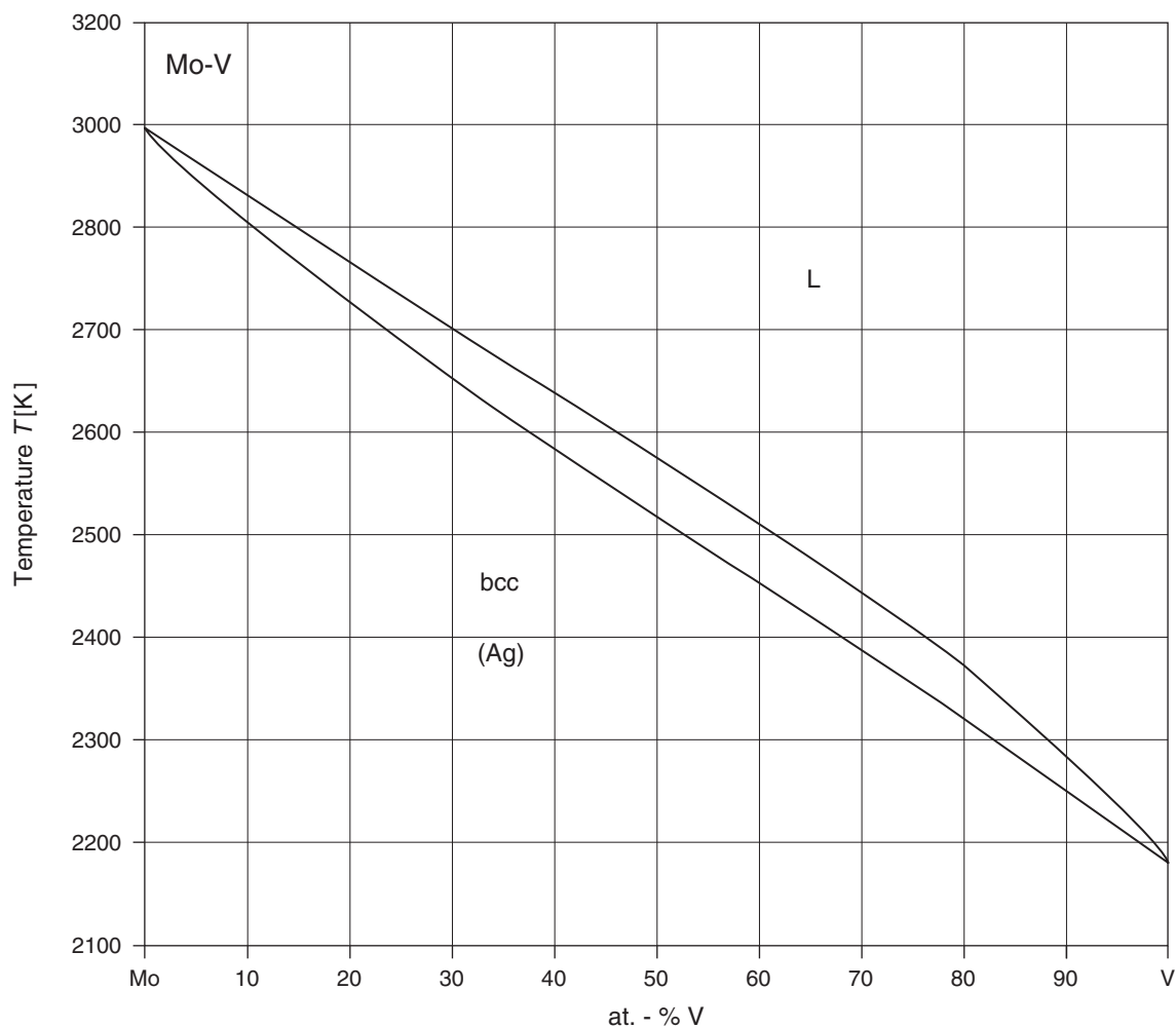
Fig. 1 Mo-V. Calculated phase diagram [99Zhe]
