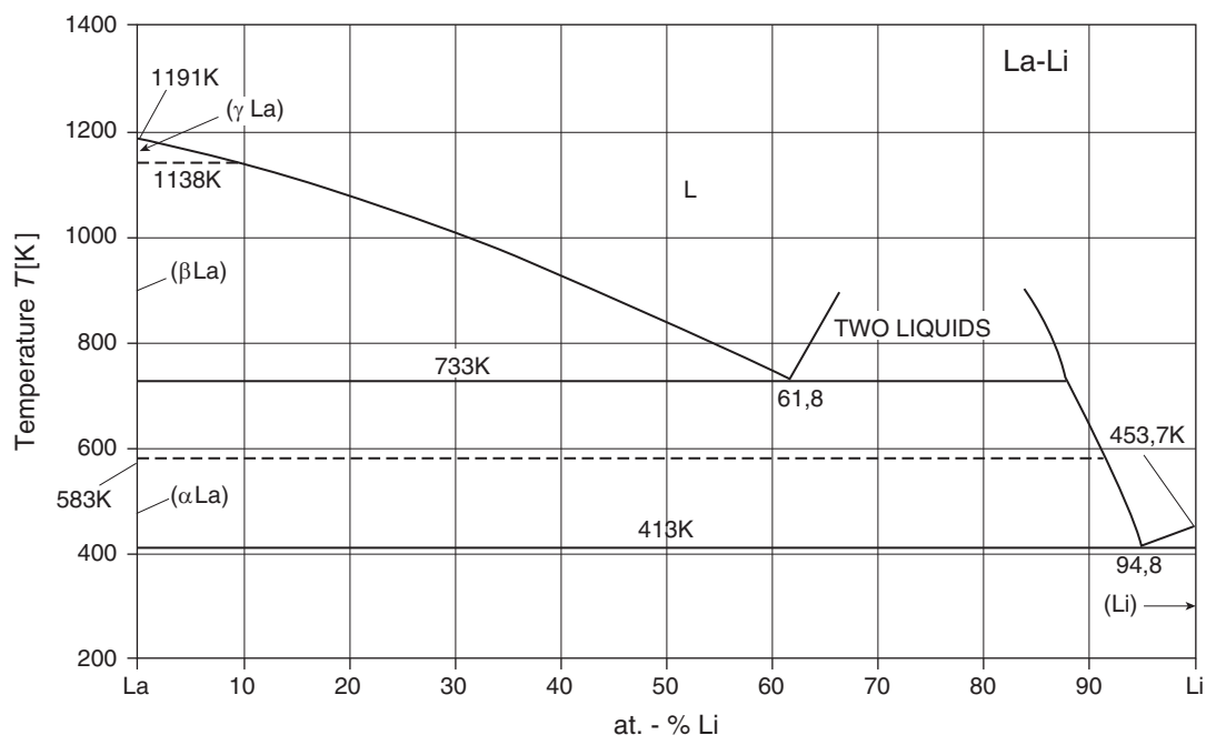
Fig. 1 La-Li. An assessed phase diagram [97Oka]
