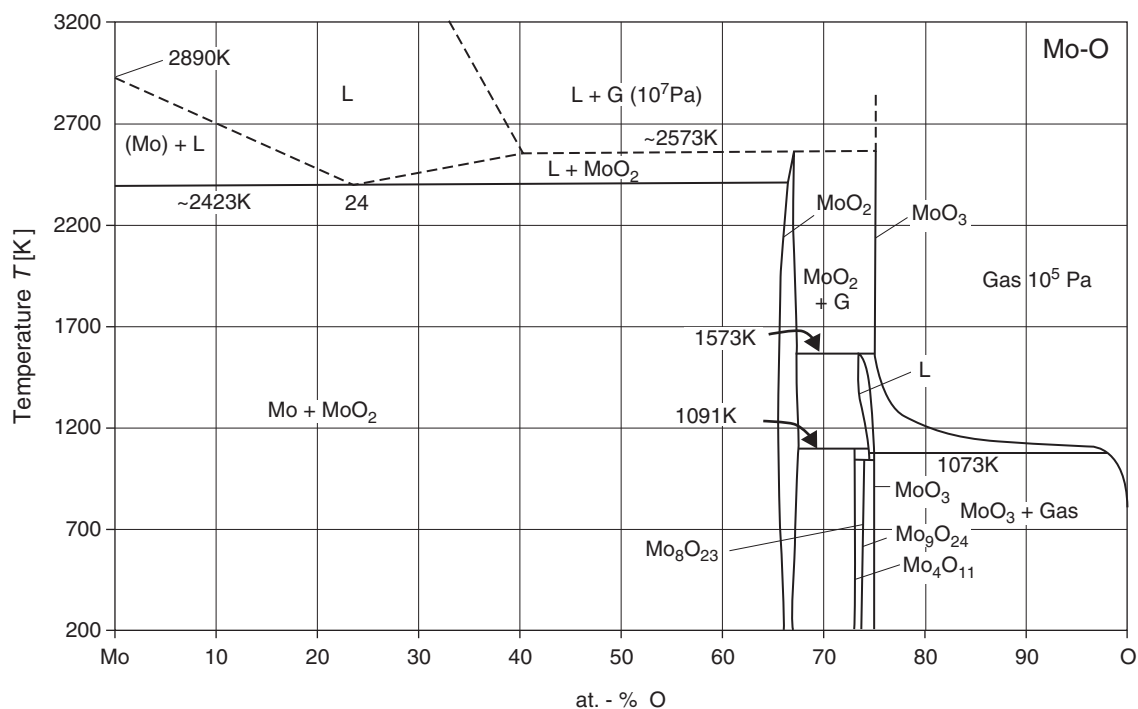
Fig. 1 Mo-O. Phase diagram taken from [Moffatt] (see [80Bre])
