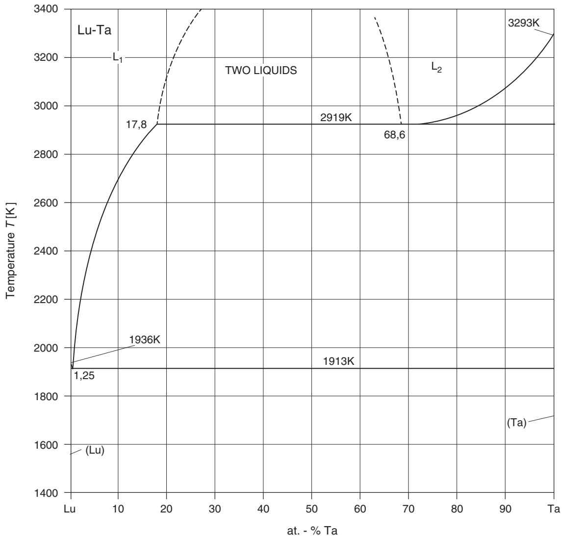
Fig. 1 Lu-Ta. Calculated phase diagram [98Gar]
