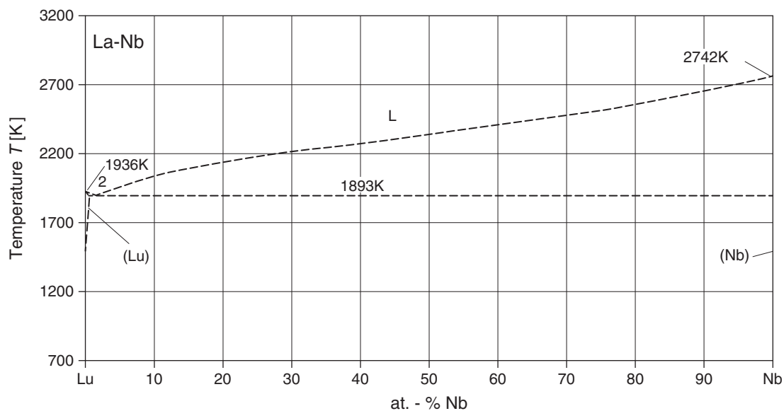
Fig. 1 Lu-Nb. Phase Diagram constructed by [99Oka]
