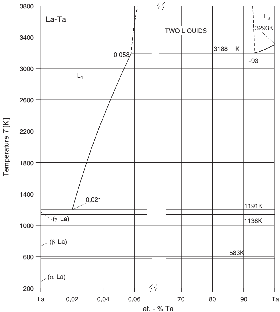
Fig. 1 La-Ta. An assessed phase diagram [98Gar]
