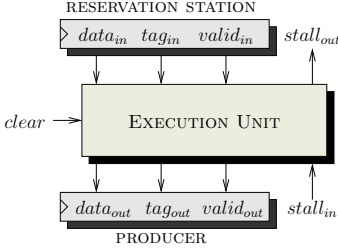
Fig. 3. Model of an execution unit
