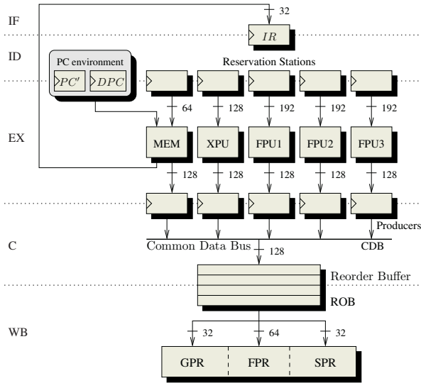
Fig. 1. Main data paths of the VAMP processor
