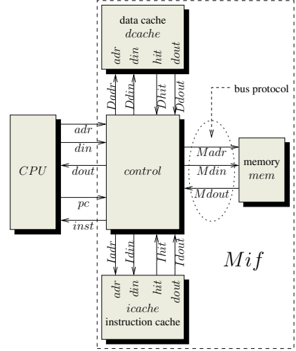
Fig. 5. Cache memory interface
