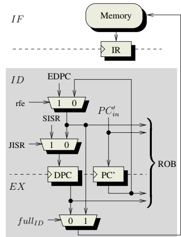
Fig. 4. VAMP PC Environment
