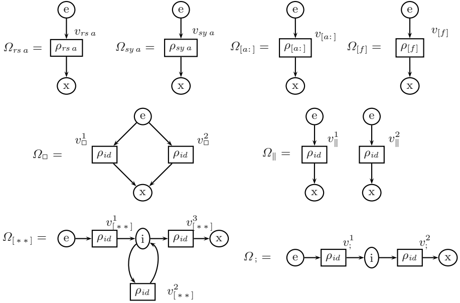
Fig. 1. The operator s-boxes for sPBC
