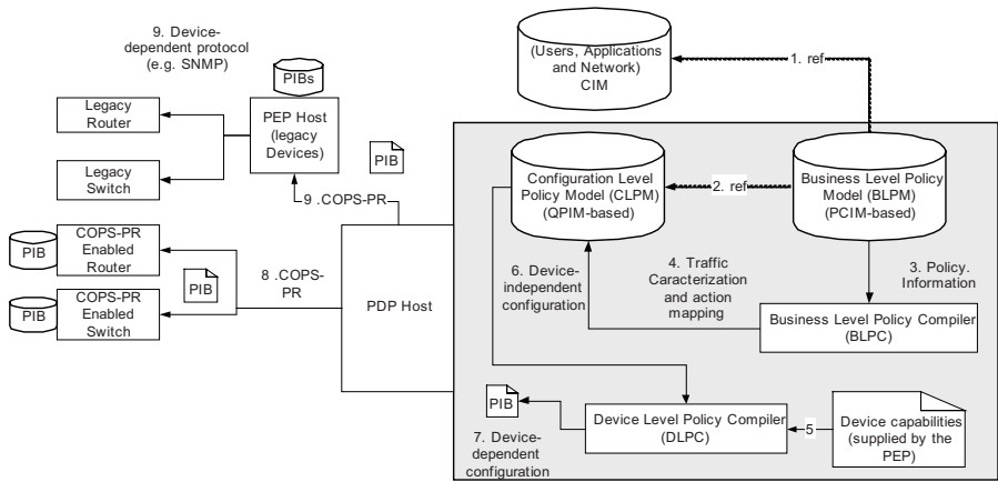
Fig. 1. Framework overview.
