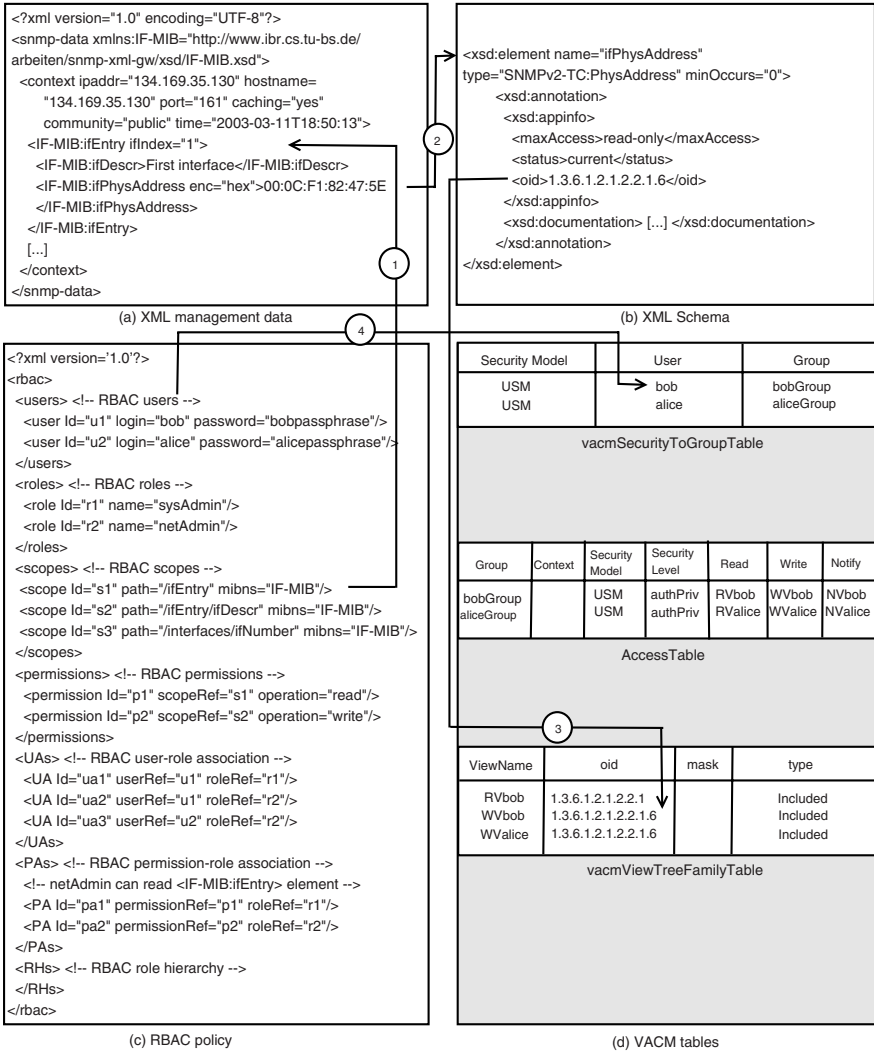
Fig. 2. RBAC/VACM mapping
