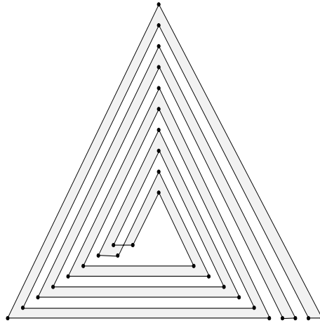
Fig. 2. A polygon with one crossing which cannot be untangled in few moves.
