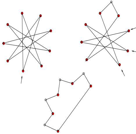
Fig. 1. For a star-polygon P with n vertices, we have f(P) = \frac{n+1}{2}
