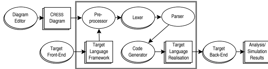
Fig. 8. CRESS Toolset
