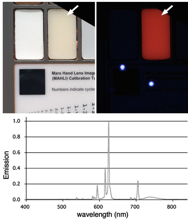
Fig. 12 Fluorescent swatch on the MAHLI calibration target. Top left: Swatch ( arrow ) under visible light. Top right: Swatch ( arrow ) under MAHLI 365 nm UV LED illumination; the two bright spots are reflections off the bar target of the violet portion of the UV LED output. Bottom: Fluorescence spectrum of the SpectraFluor Red pigment. The images of the MAHLI calibration target were acquired during rover system thermal testing on 14 March 2011. The large, dark square at top left is 8 by 8 mm
