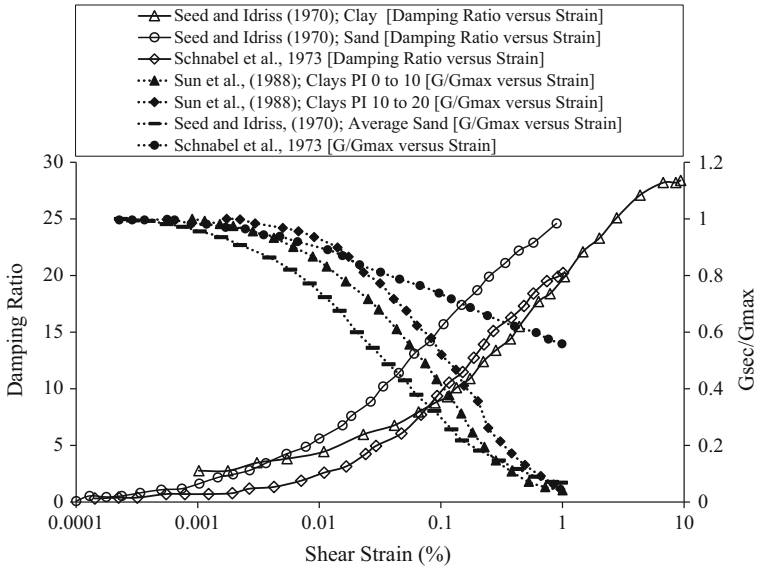
Fig. 2 Dynamic properties of selected soils
