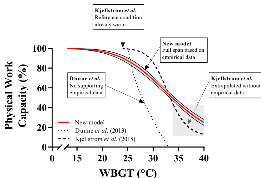
Fig. 6 The relationship between PWC and WBGT for past models and the new model. Deriving relations based on work/rest ratios (dotted line, Dunne et al. (2013)) or from past field data (dashed line, Kjellstrom et al. 2018) underestimate the effect of moderate heat stress and overestimate the effects of extreme heat stress, resulting in unrealistically steep declines in PWC. The red line shows the new model, based on Fig. 2a, where we
