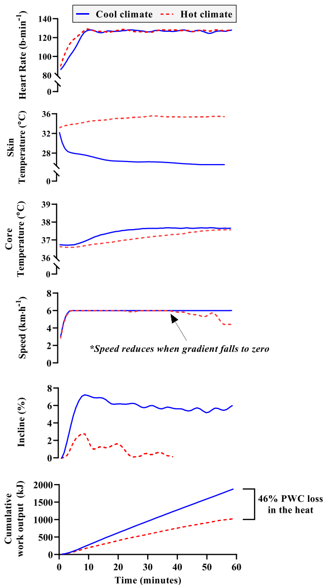
Fig. 1 Fixed heart rate protocol measures how climatic heat impacts work capacity. Field studies demonstrate that individuals work at a similar heart rate despite changes in climatic heat due to adjustments in pacing. Although the heart rate profile is not different between conditions, heat stress causes a substantial increase in skin temperature, causing dramatic reductions in overall energy generated. Core (rectal) temperature responses in the early phase of the exposures are driven primarily by metabolic heat production (work rate). Changes to cumulative energy expenditure were used to calculate physical work capacity (PWC). Example data is shown for a representative participant for the reference condition (15°C, 50% humidity, solid blue line) and a hot condition (40°C, 20% humidity, dashed red line)
