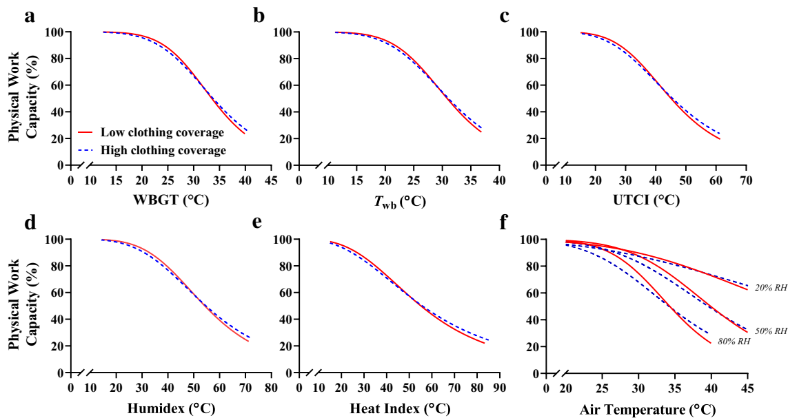
Fig. 4 Clothing-specific models for physical work capacity. Models are presented based on low (red lines) or high (blue lines) levels of clothing coverage. Unlike the pooled data shown previously, the models here can be used for specific industries based on whether protective clothing is
