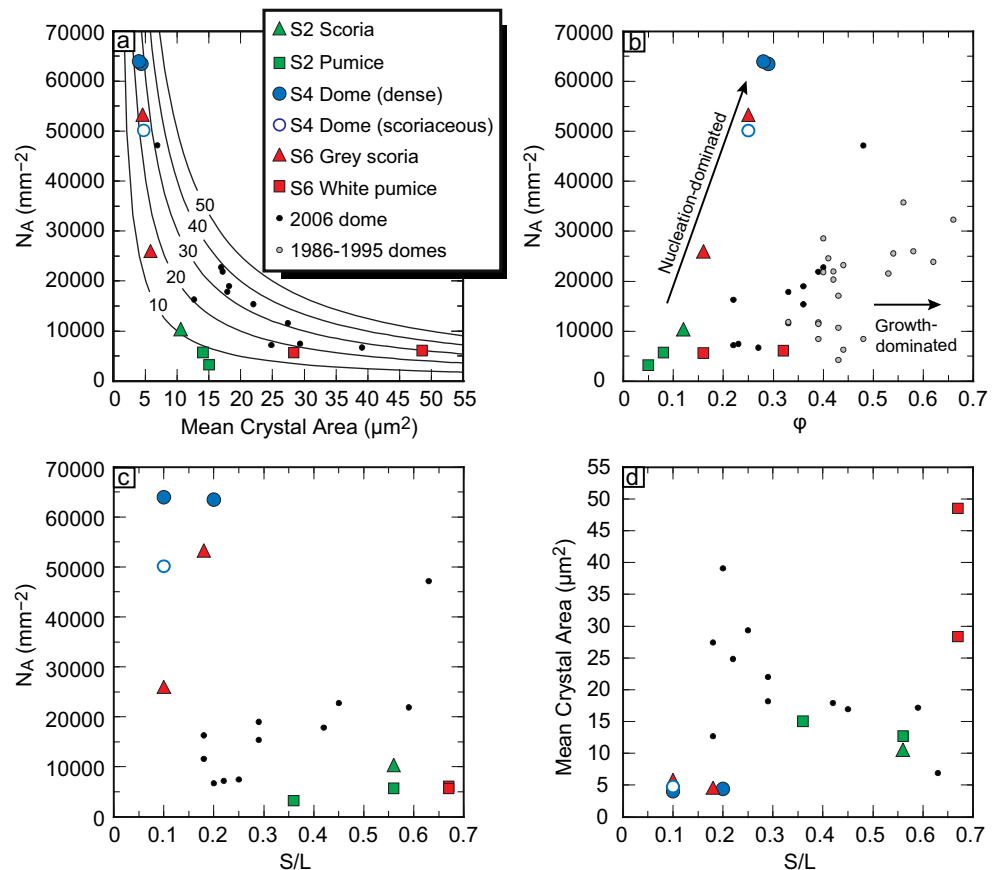
Fig. 3 Variation in textural parameters in 2010 products, plotted with those from 2006 dome products (Preece et al. 2013) for comparison. a Areal feldspar microlite number density ( N_A mm -2 ) vs. mean crystal area ( \mu\text{m}^2 ), with solid lines indicating modelled microlite crystallinity at a particular N_A and crystal size. b Areal feldspar microlite number density ( N_A mm -2 ) vs. feldspar microlite crystallinity ( \varphi ) including data from other recent (1986–1995) effusive dome-forming eruptions (Hammer et al. 2000). c Areal feldspar microlite number density ( N_A mm -2 ) vs. short/long axis ( S/L ). d Mean crystal area ( \mu\text{m}^2 ) vs. S/L
