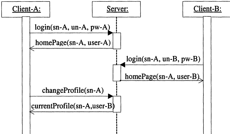
Figure 3. Session hijacking scenario
