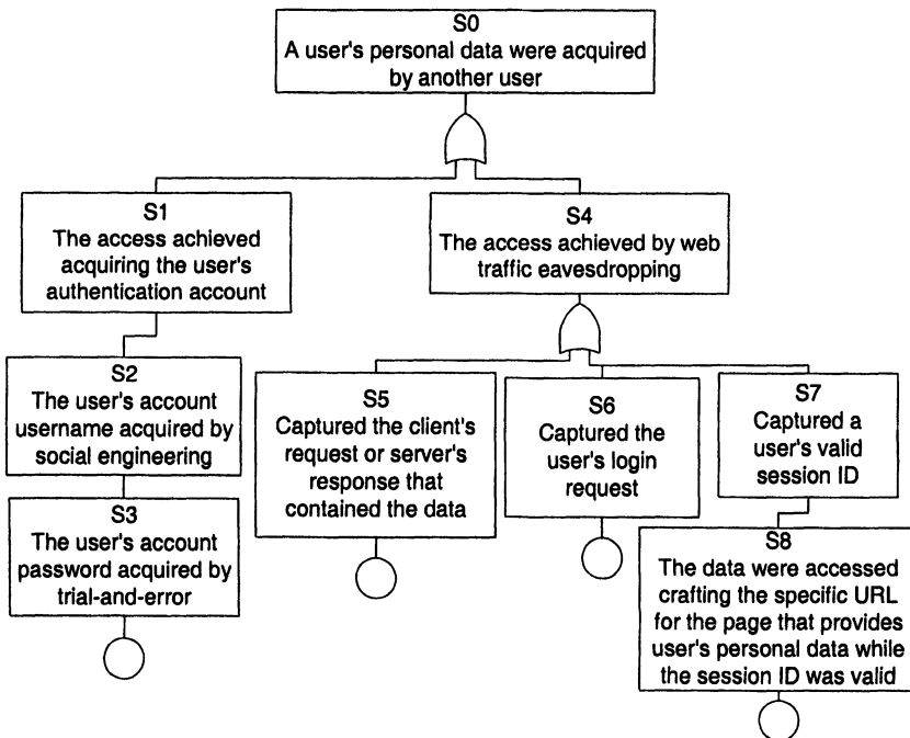
Figure 5. A Fault Tree example for capturing confidential data
